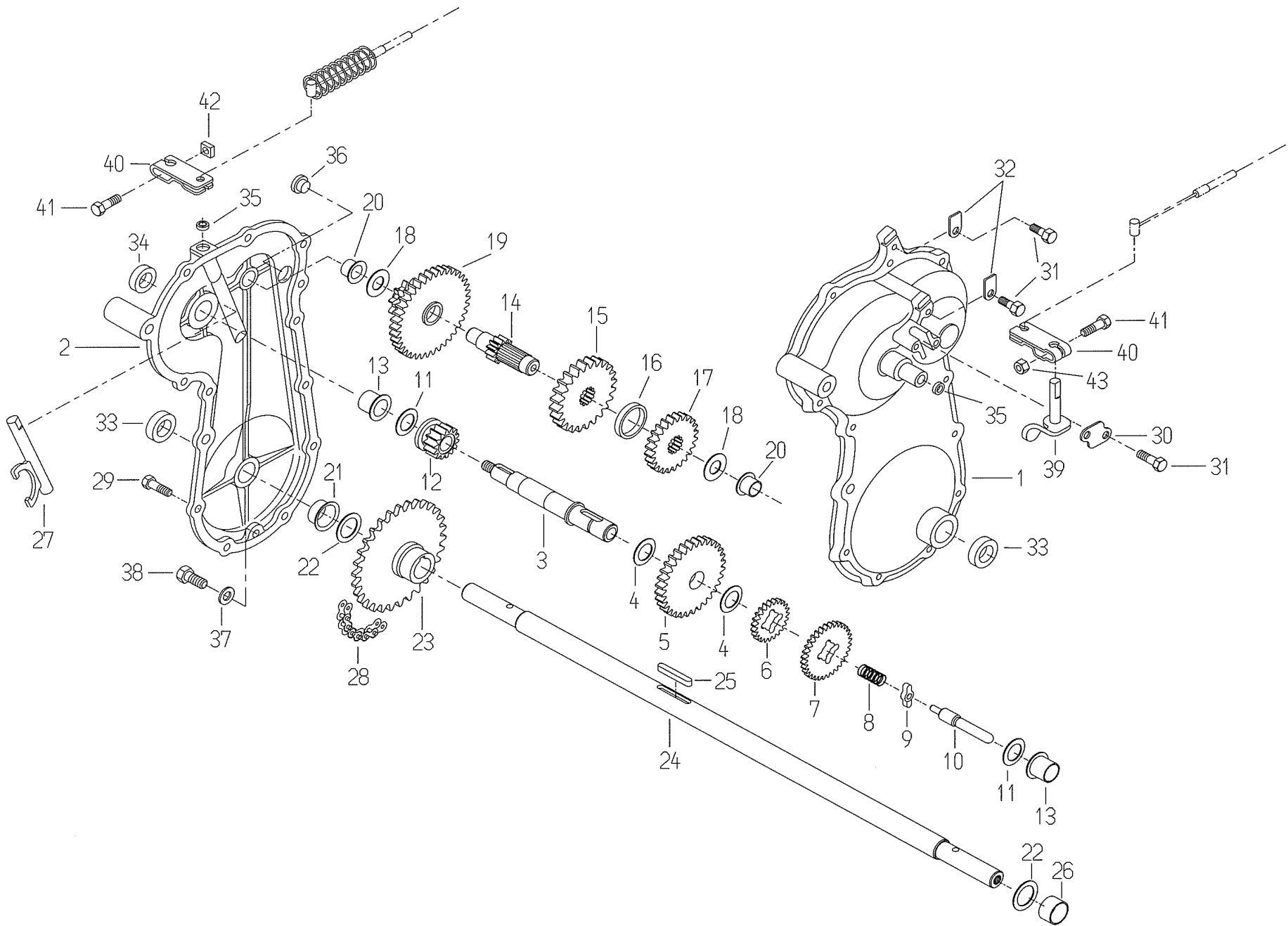
Fig. 2 TRANSMISSION
