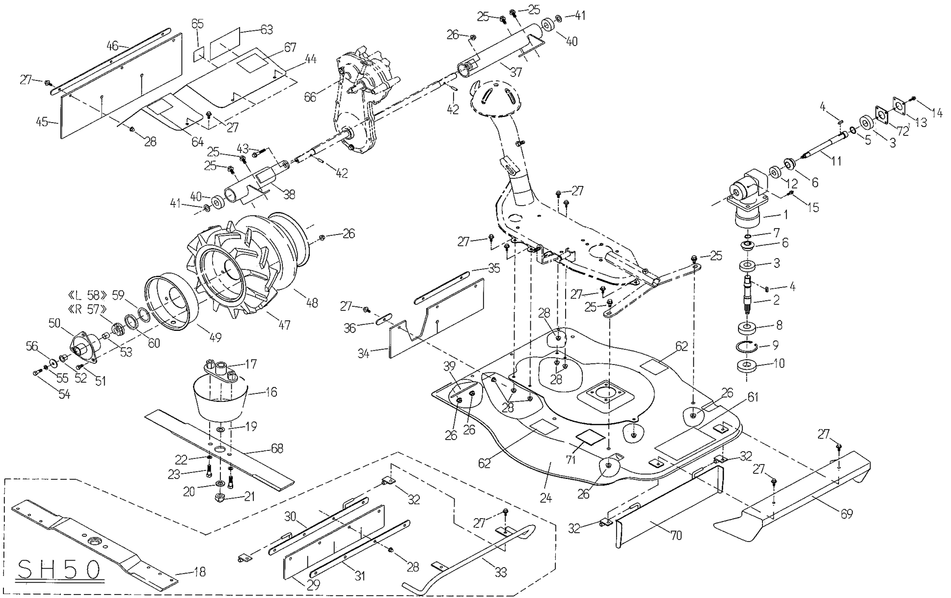
Fig. 4 GEAR BOX . ROTARY COVER & TIRE
