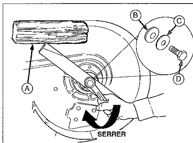
Figure 24. Installation de la lame
