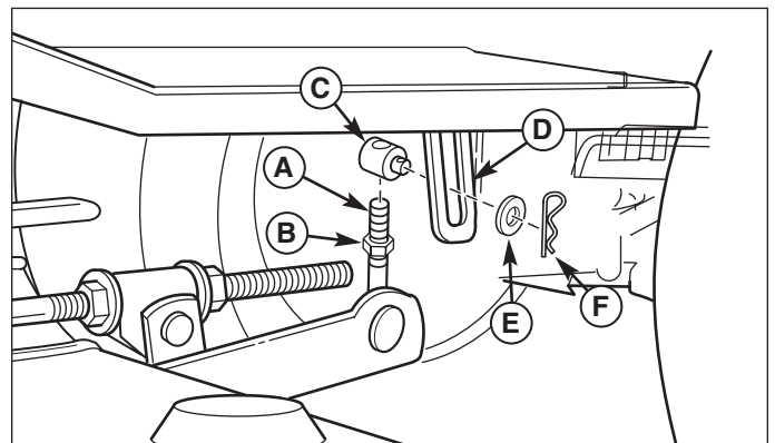
Figure 57. Broadmoor Cutting Height Adjustment
