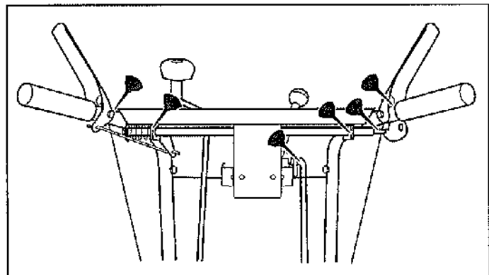
Figure 17. Lubrification de la commande Free Hand
