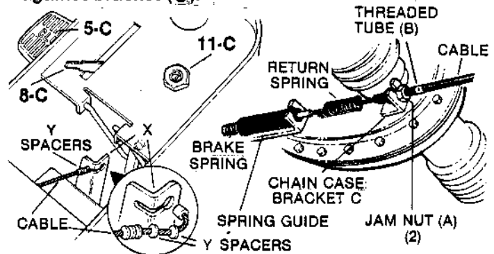
FIG. 12 - CLUTCH/BRAKE ADJUSTMENT
