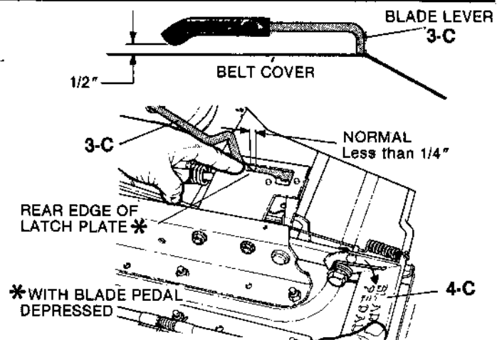
FIG. 10 - BLADE LEVER TRAVEL
