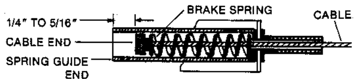
FIG. 12 - CLUTCH/BRAKE ADJUSTMENT
