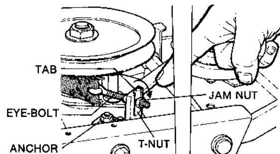
FIG. 11 - BLADE BRAKE ADJUSTMENT
