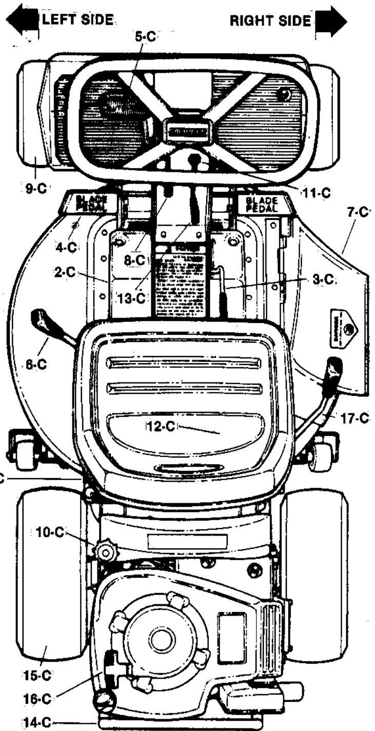
FIG. 1 - LOCATION OF CONTROLS/FEATURES
