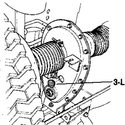
FIG. 5 - CHAIN CASE
