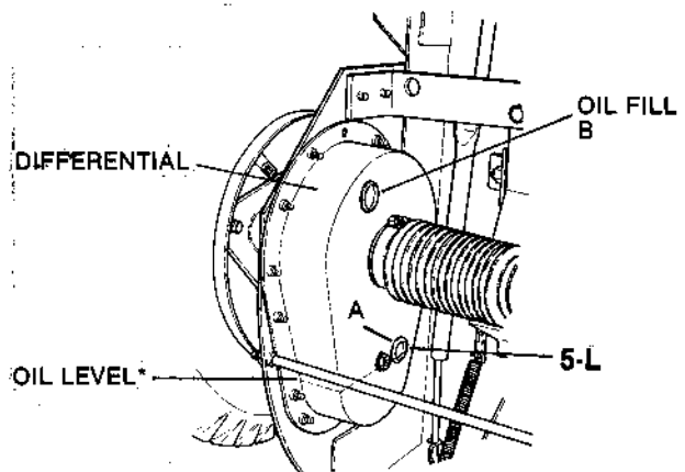
FIG. 4 - DIFFERENTIAL LUBE LEVEL
