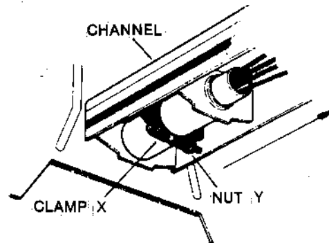
FIG. 8 - TUBE CLAMP
